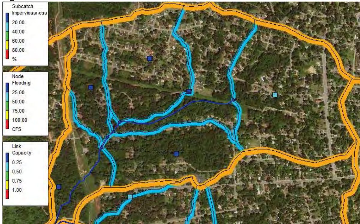
Figure 6.60 SW-L SWMM Model
