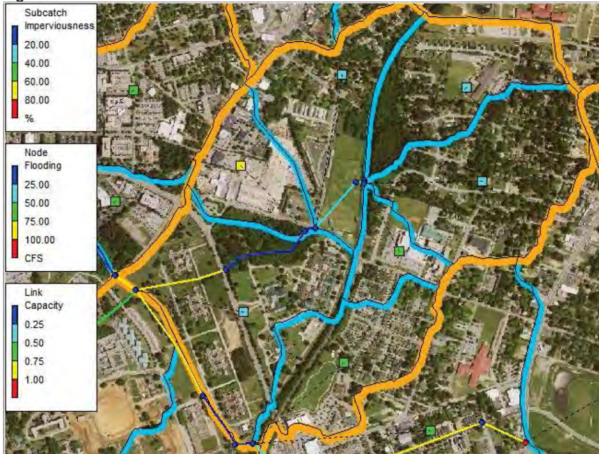
Figure 6.25 SW-G SWMM Model
